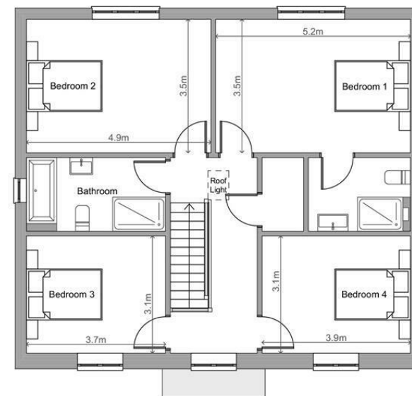
First Floor 1:100
