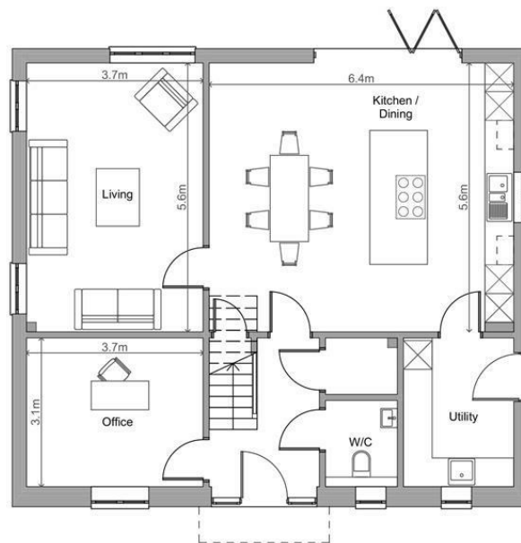
Ground Floor 1:100
